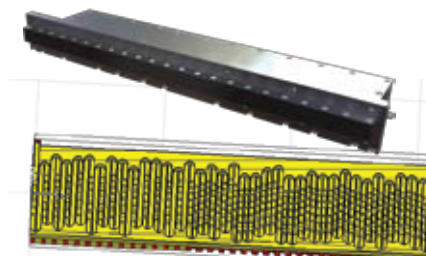
Ku-band steerable antenna which incorporates serpentine waveguide distribution/coupler array
