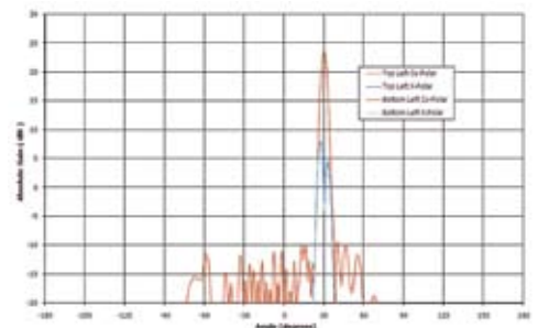
Antenna pattern at one frequency showing 30° offset and very low sidelobes
